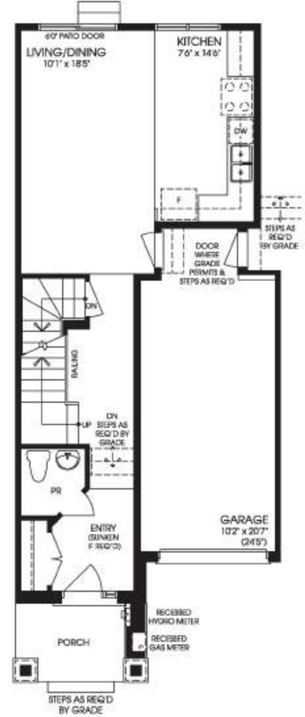
MAIN FLOOR ELEVATION 'A2'
