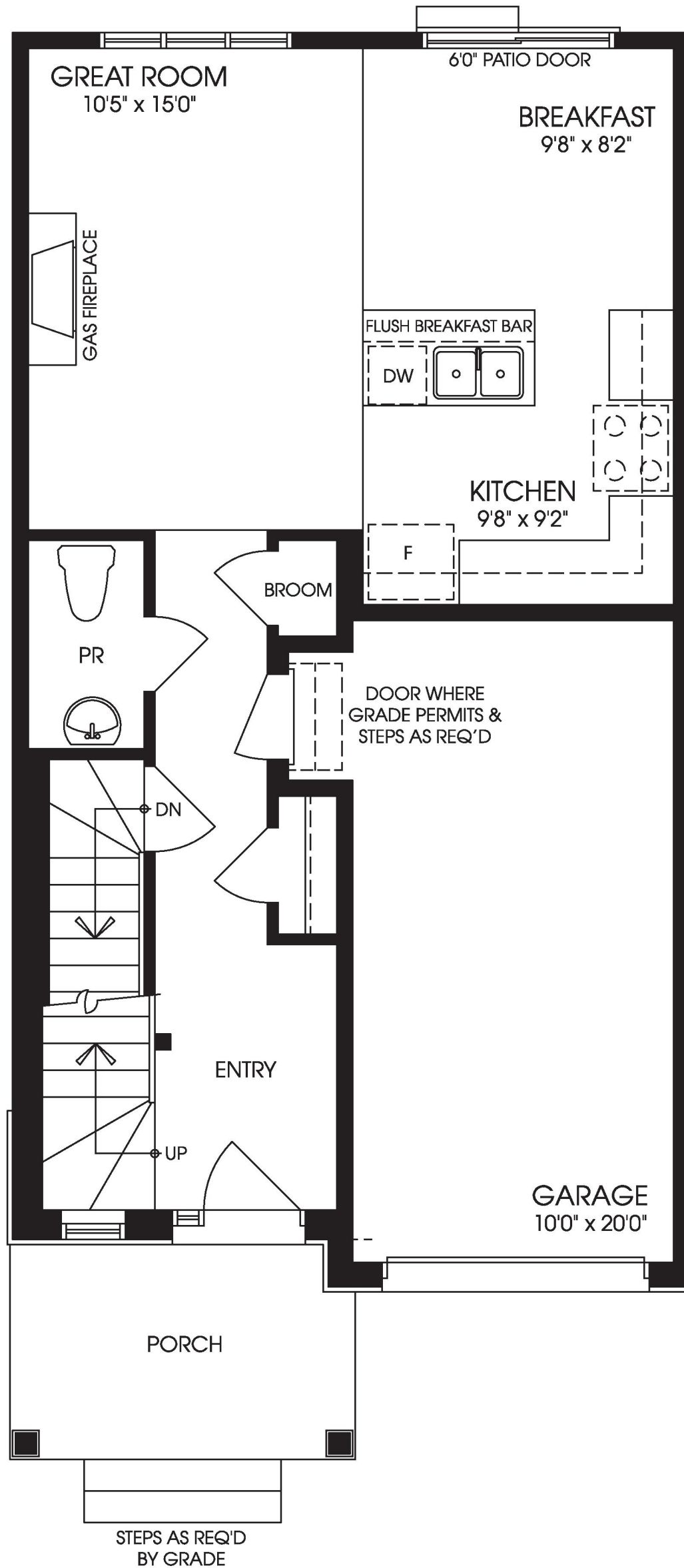
MAIN FLOOR ELEVATION 'A1'
