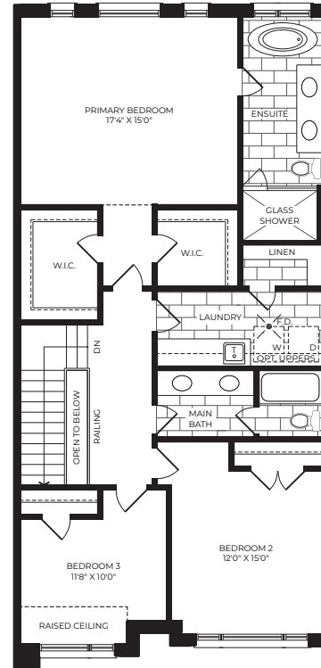
ELEVATION B Second Floor
