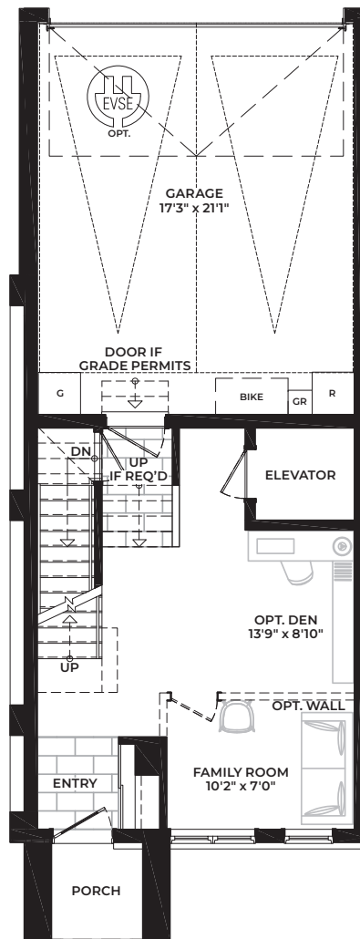
B1 B Porch End Opt. Elevator GROUND FLOOR
