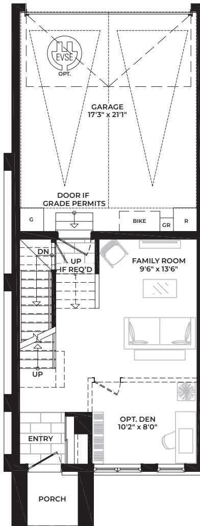
B1 B Porch End GROUND FLOOR
