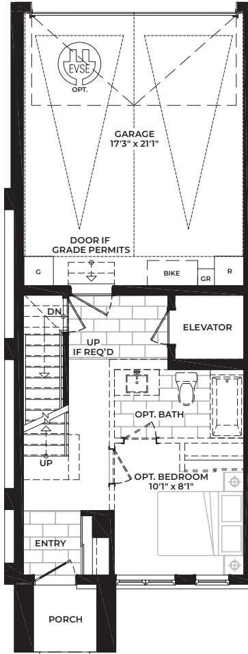
B1 B Porch End. Opt. Elevator & Opt. Bedroom GROUND FLOOR
