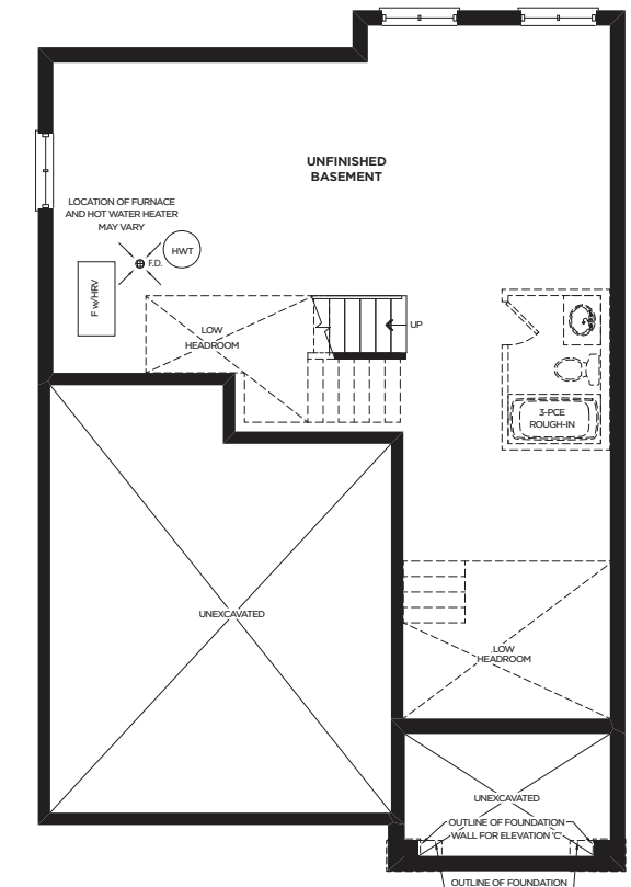
BASEMENT ELEVATION A, B & C
