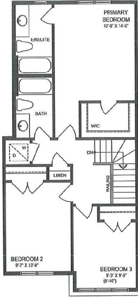
SECOND FLOOR ELEVATION 'A1'
