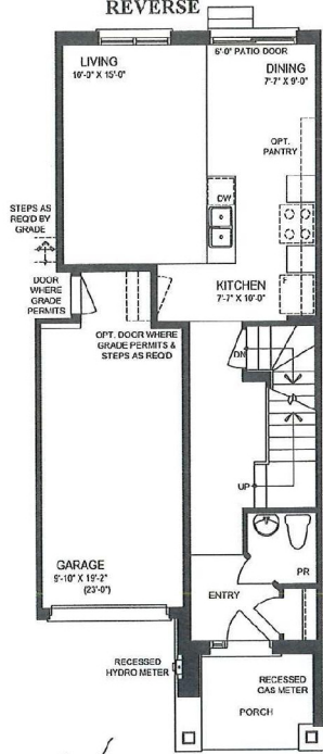
MAIN FLOOR ELEVATIONS 'A1' & 'A2'
